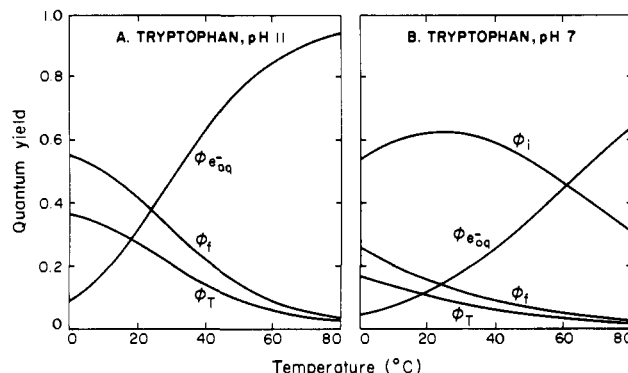
Figure 6. Calculated quantum yields of fluorescence ( \phi_f ), intersystem crossing ( \phi_{ic} ), and intramolecular quenching ( \phi_i ) for aqueous tryptophan at pH 7 and 11, as a function of temperature.
