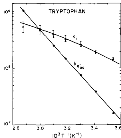
Figure 4. Temperature dependence of the rates of photoionization k_{e_{aq}^-} and intramolecular quenching k_i for aqueous tryptophan, plotted in the form \ln k vs. T^{-1} . The solid lines are the best fits of the data to eq 6 and 8, respectively.
